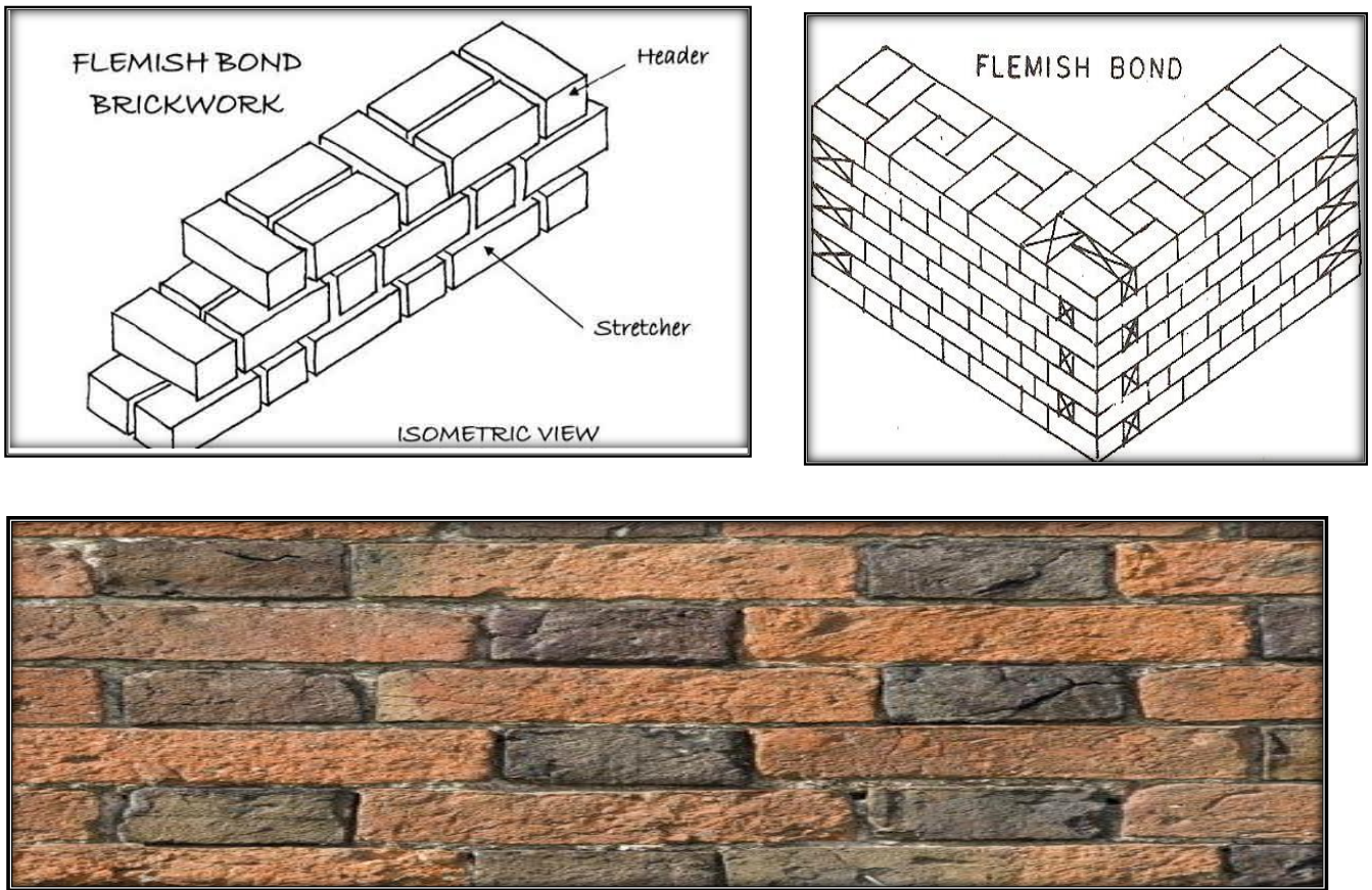
Figure 10: Flemish Bond
