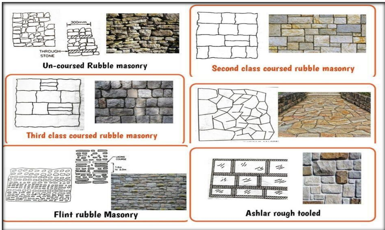
Figure 11: Stone Masonry
