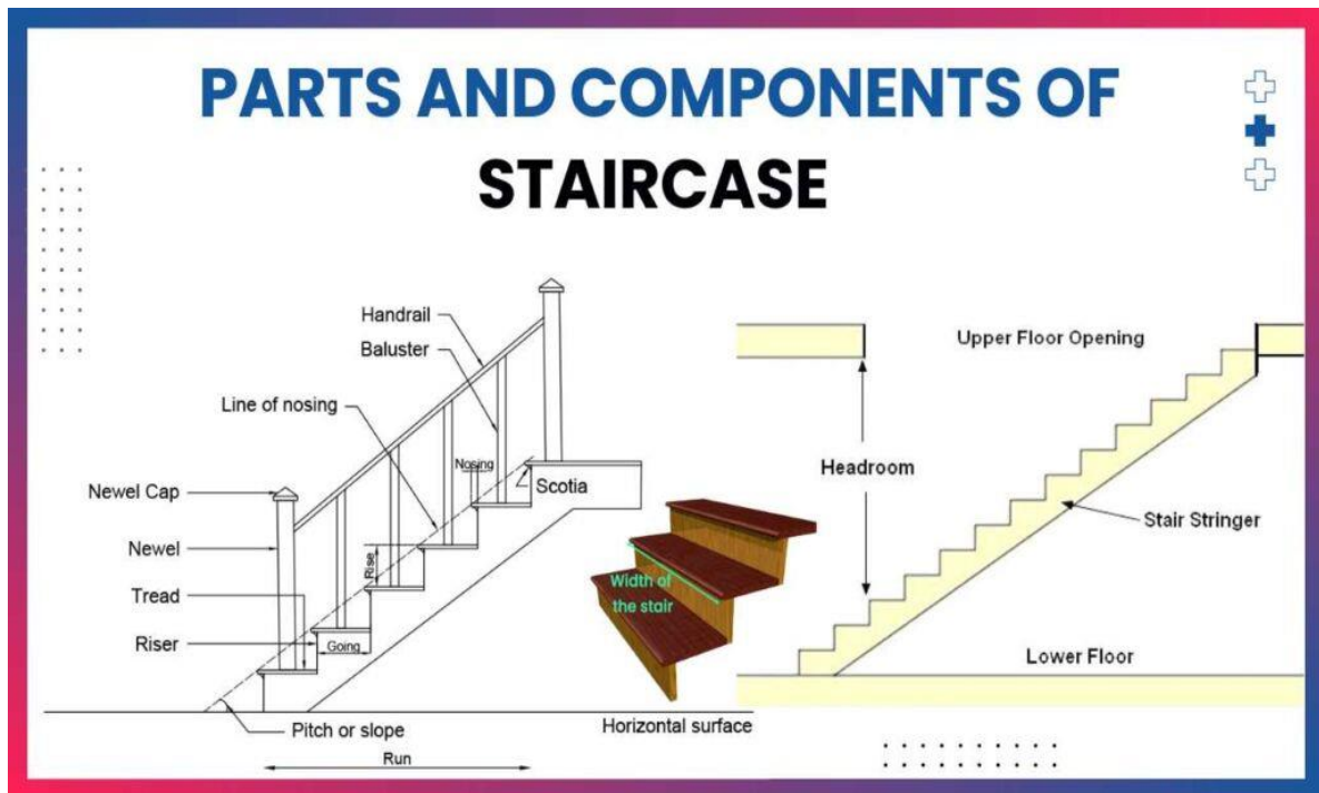
Figure 13: component parts of staircase.
