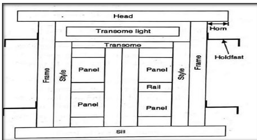
Figure 14: components Parts of Doors and windows
