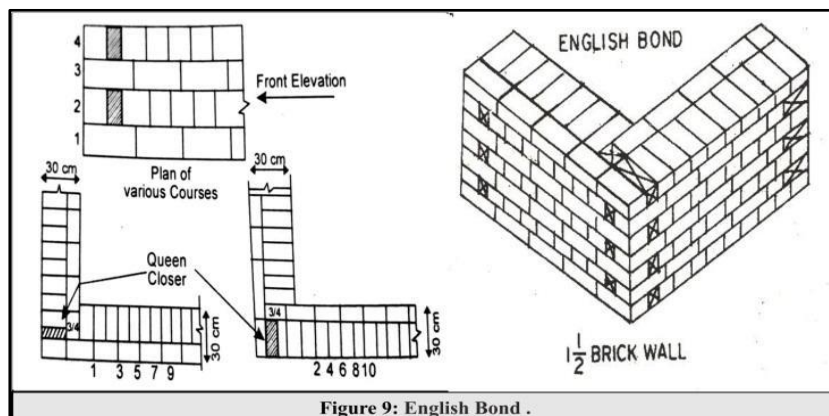
Figure 9: English Bond .
