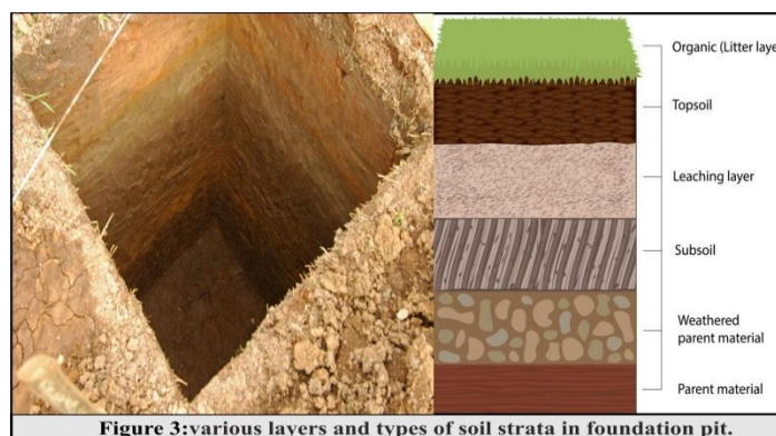
Figure 3:various layers and types of soil strata in foundation pit.
